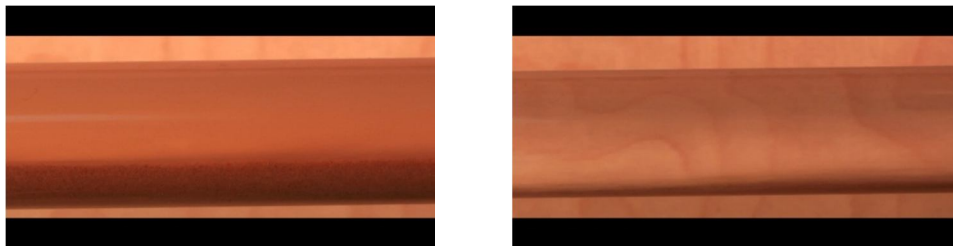
Figure 12: Pick-up velocity reached at V_1 = 0.70 m/s for 10% sand concentration by volume (side view)
