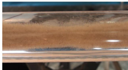
Large connected sand dunes ( V_1 = 0.40 m/s)
