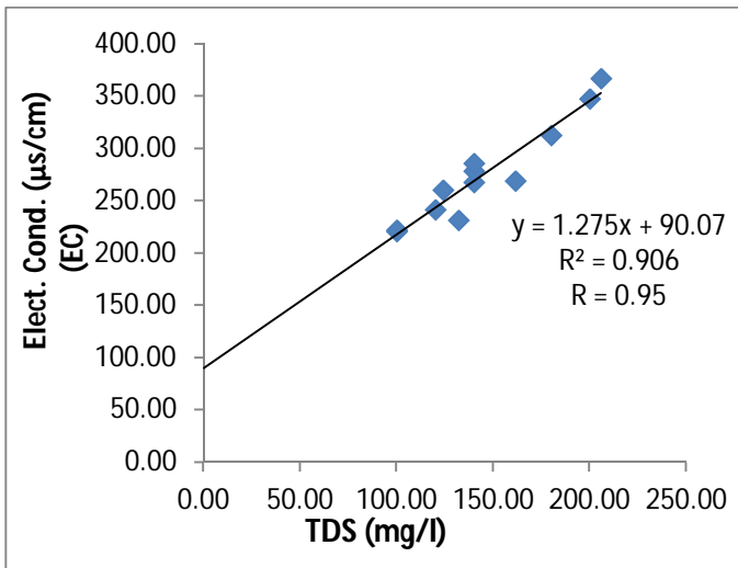
Figure 3a. Regression of EC on TDS
